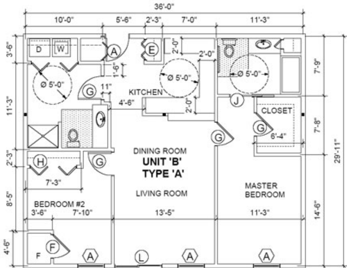
TWO BEDROOM TYPE 'A' - 1040 SF
